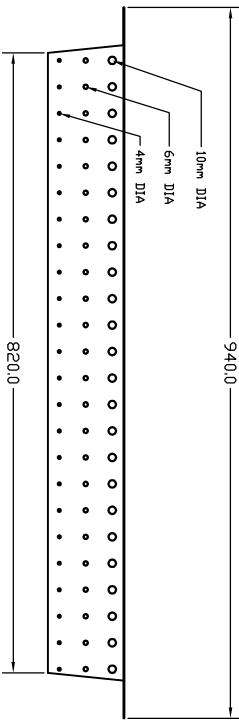
FRONT VIEW
